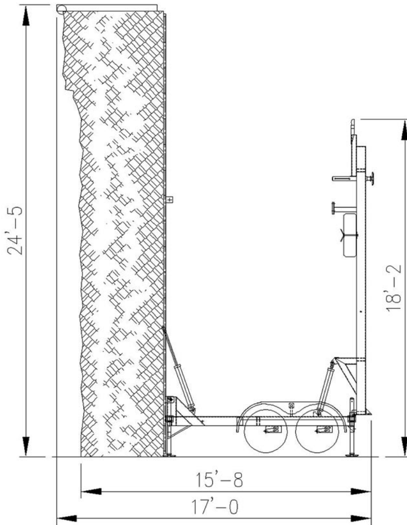
24' DAR STANDING SIDE VIEW
